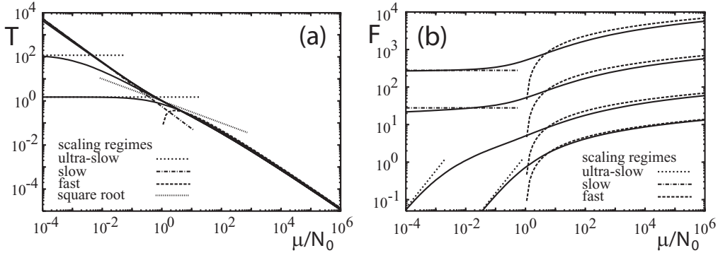
Fig. 4 – (a) Mean cluster lifetime T and (b) mean rupture force F = \mu T for the case \gamma = 1 as a function of \mu/N_0 for N_t = 2, 10, 10^2 and 10^3 . In (a), the curves for the two larger clusters are nearly identical.
