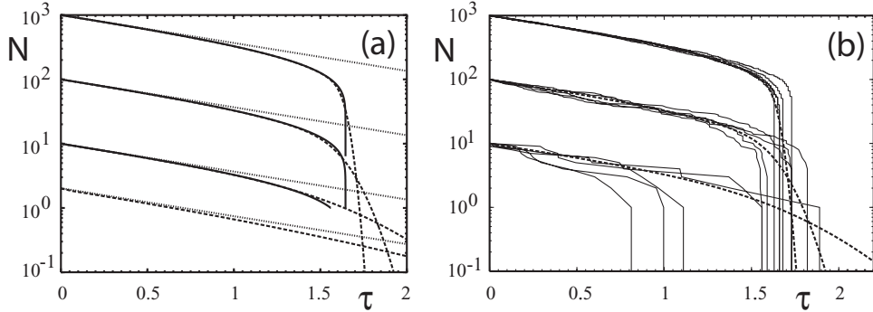
Fig. 1 – (a) Mean number of closed bonds N as a function of time \tau for the case of vanishing rebinding, \gamma = 0 , for \mu/N_0 = 0.1 and N_t = N_0 = 2, 10, 10^2 and 10^3 . Dotted lines: initial exponential decay. Dashed lines: first moment of the Monte Carlo simulations. Solid lines: numerical integration of deterministic rate equation (not for N_t = 2 ). (b) Individual trajectories from Monte Carlo simulations in comparison with the mean (not for N_t = 2 ).
